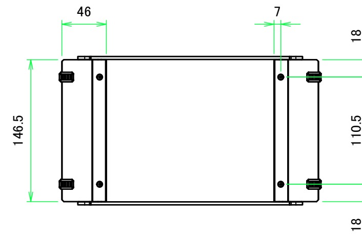
C-C (1:4)
