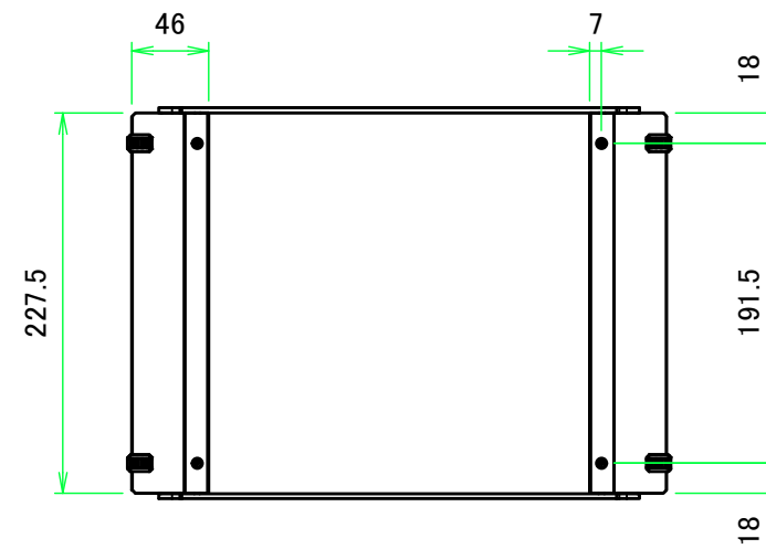
C-C (1:5)
