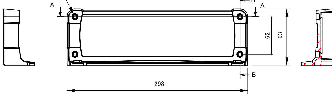
B-B (1:3)
