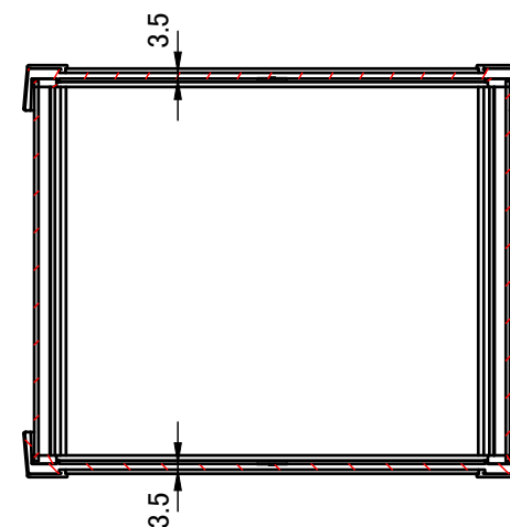
C-C (1:5)
