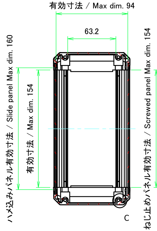
B-B (1:3)
