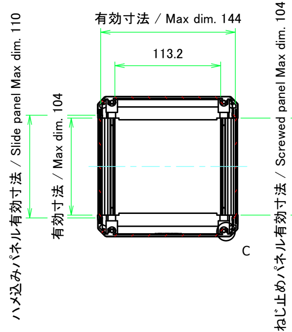
B-B (1:4)
