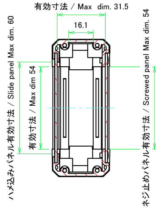
B-B (1:1.5)
