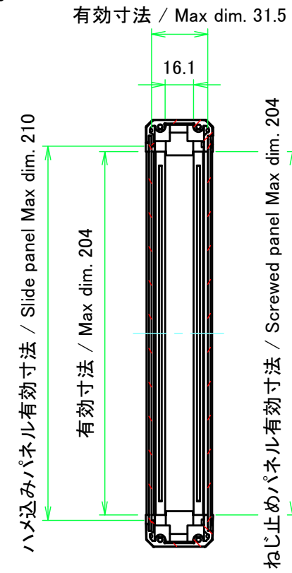
B-B (1:3)
