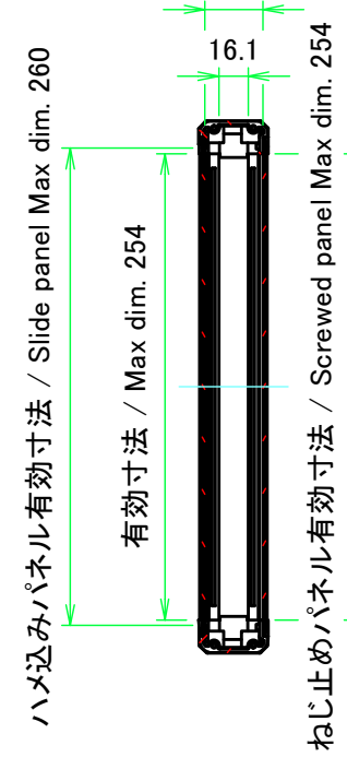
B-B (1:4.5)
