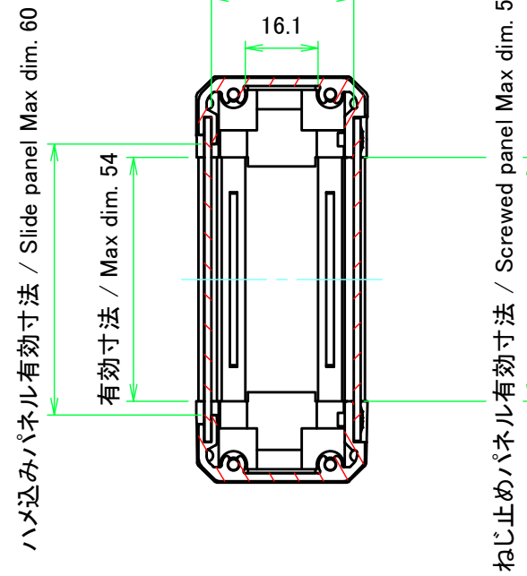
B-B (1:1.5)
