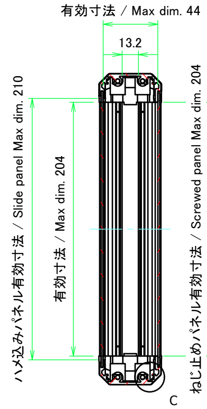
B-B (1:3)
