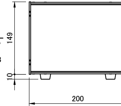
C view
