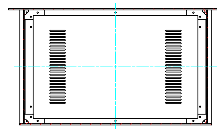
B-B (1:5)
