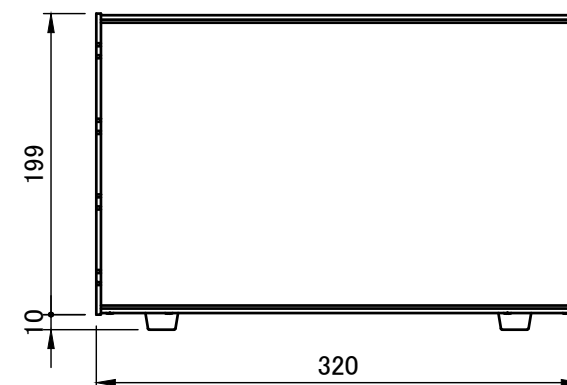
B-B (1:5)
