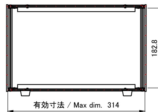
C view
