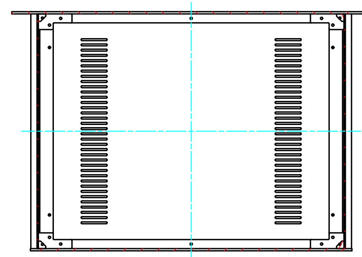
B-B (1:5)
