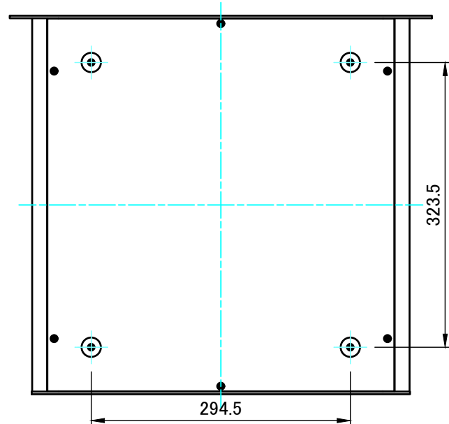
F view
