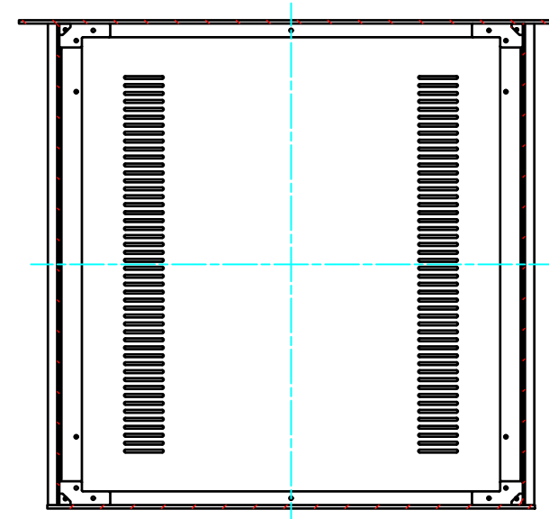
B-B (1:6)
