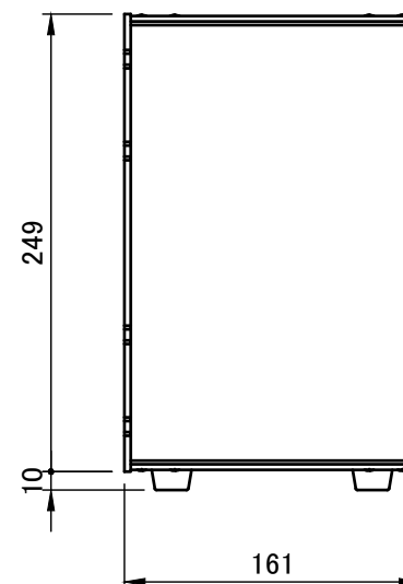
C view
