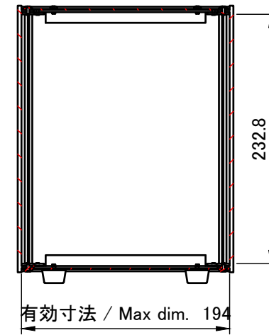
C view
