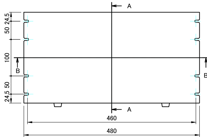
A view
