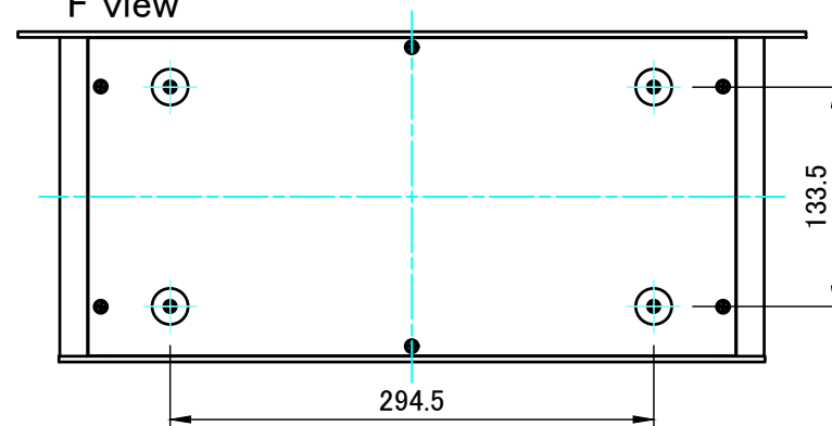
F view
