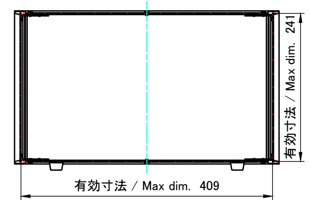
C-C (1:6)
