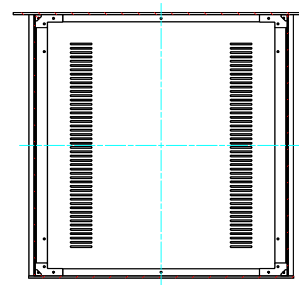
B-B (1:6)
