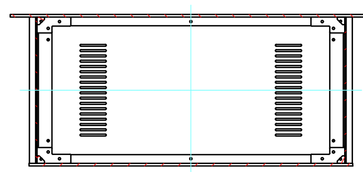
B-B (1:5)
