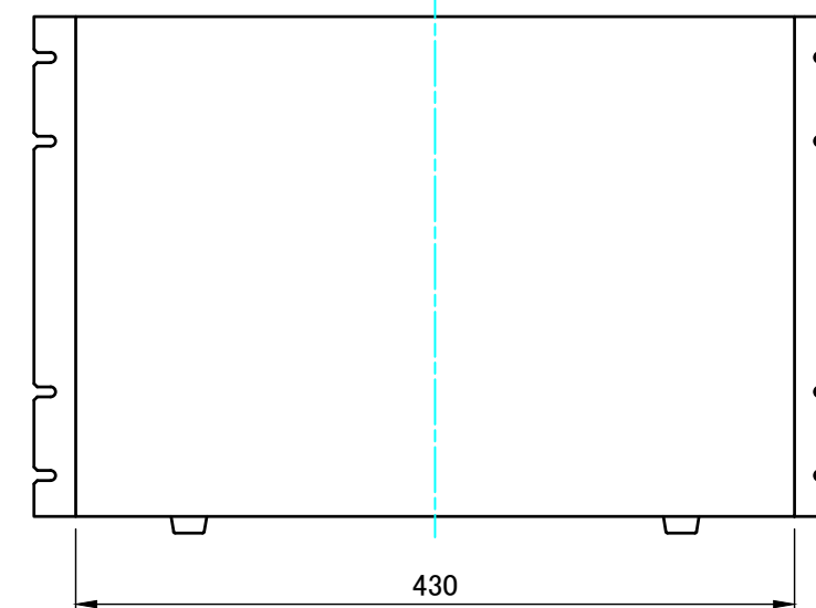
B view
