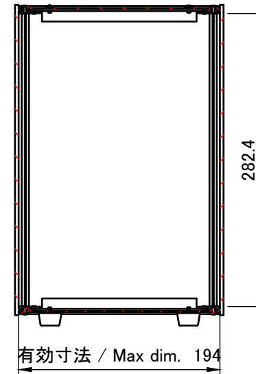
C view
