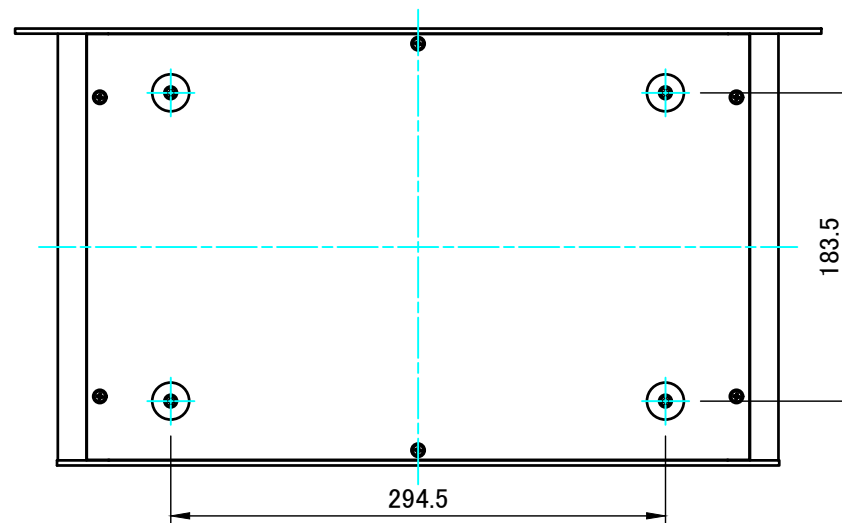
F view
