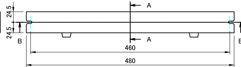
A view
