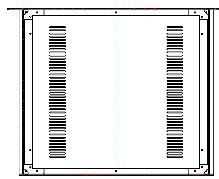
B-B (1:5)
