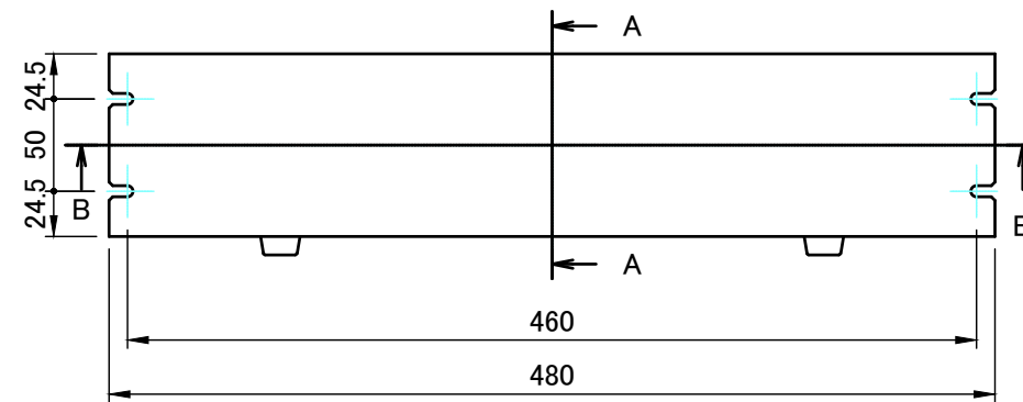
A view
