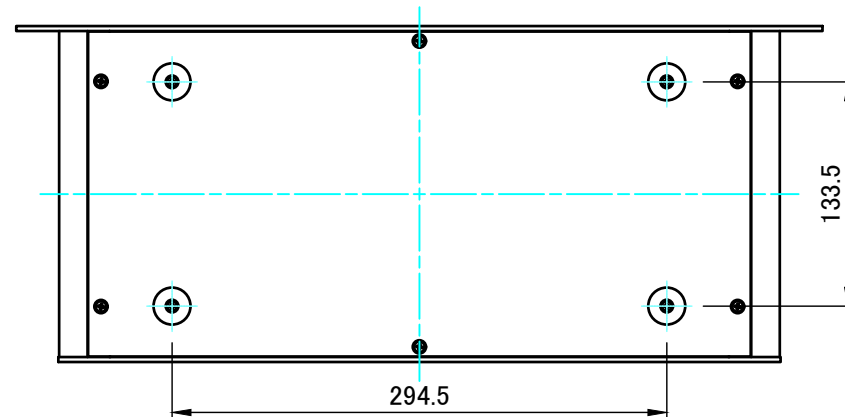
F view
