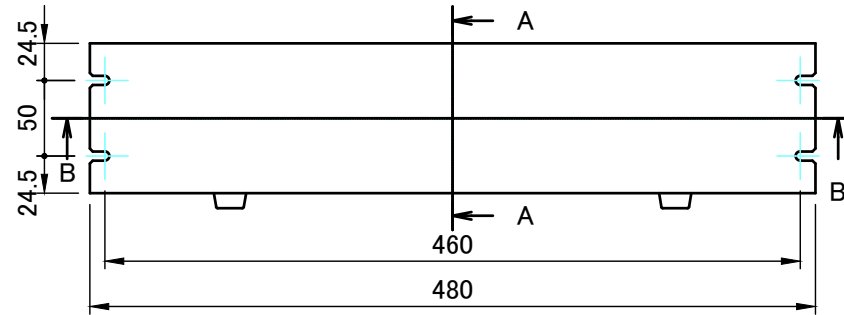
A view
