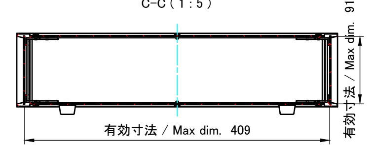
C-C (1:5)
