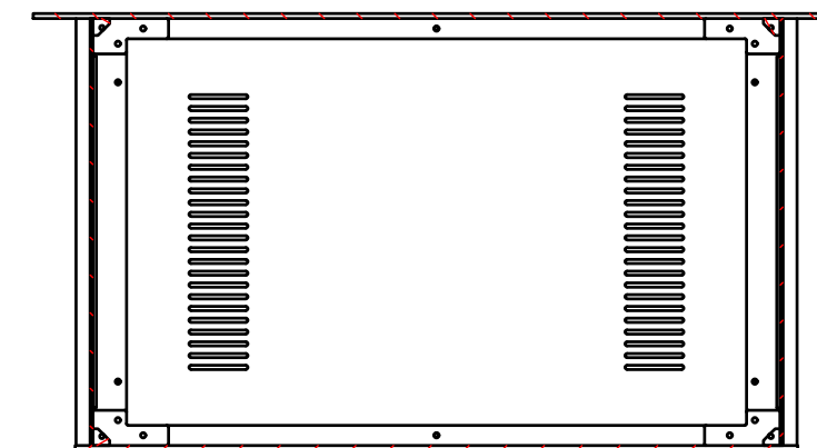
B-B (1:5)
