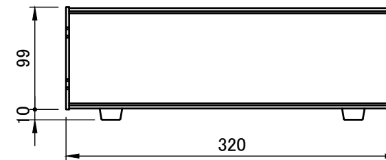
C view
