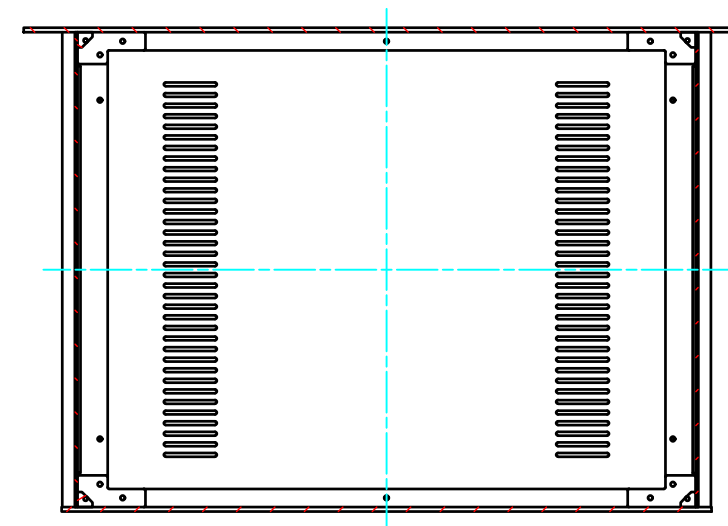
B-B (1:5)
