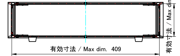
C-C (1:5)
