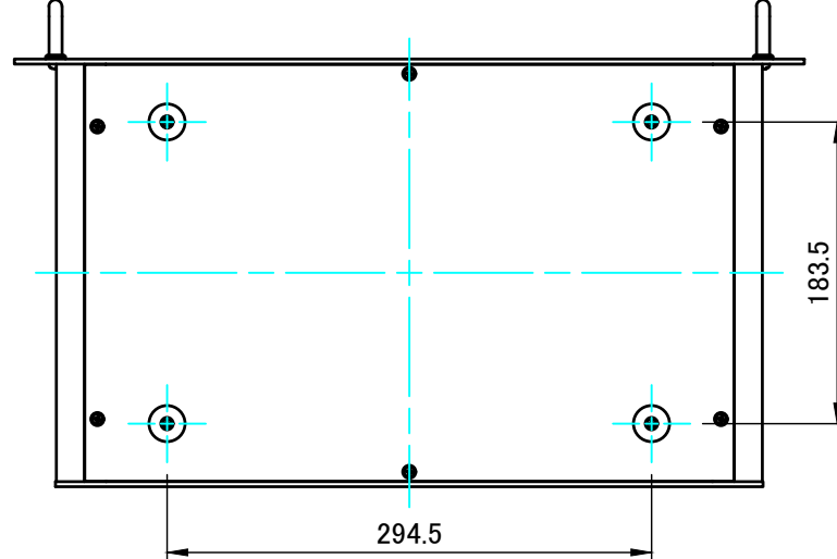
F view
