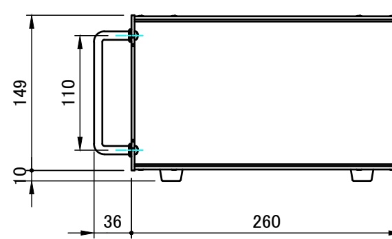
C view
