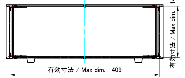
C-C (1:5)
