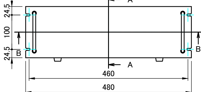
F view
