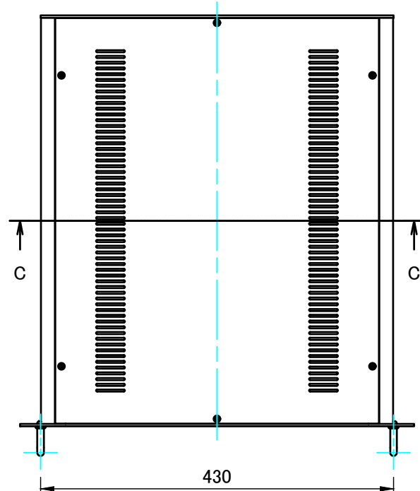
E view
