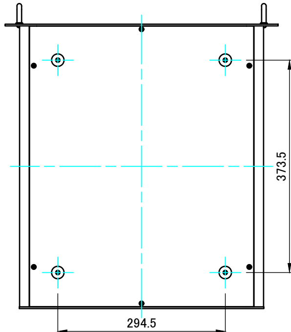
F view
