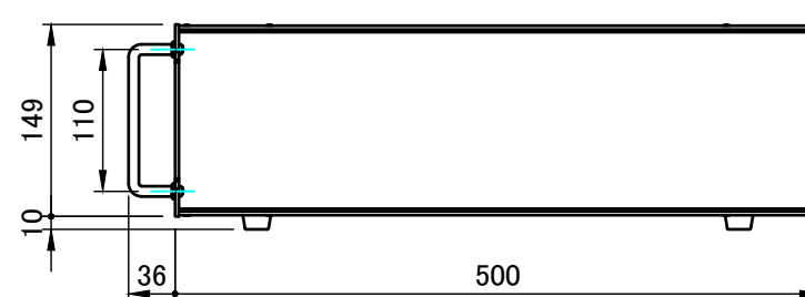
C view
