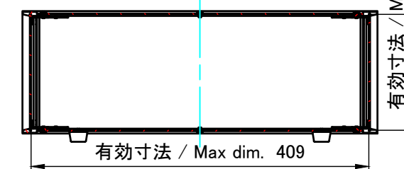
C-C (1:6.5)
