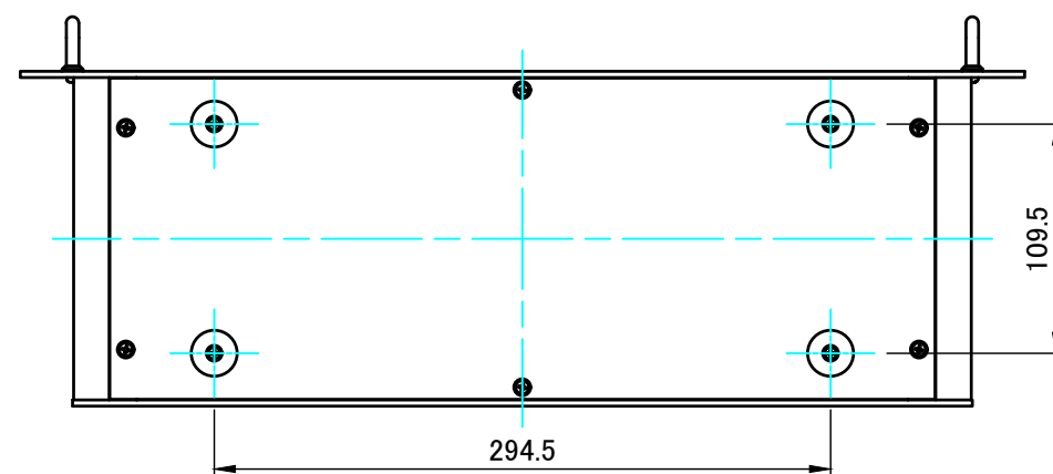
F view
