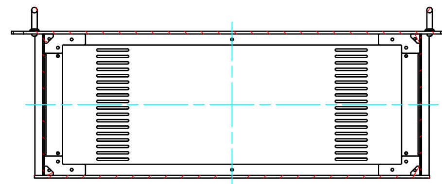
B-B (1:4)
