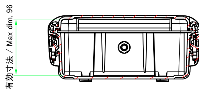
B-B (1:4)
