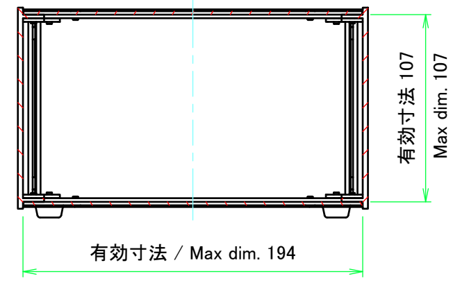
C-C (1:3)
