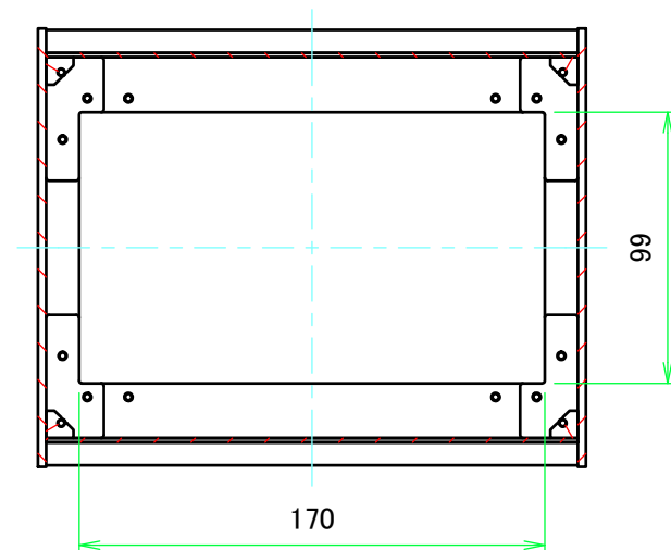
B-B (1:3)
