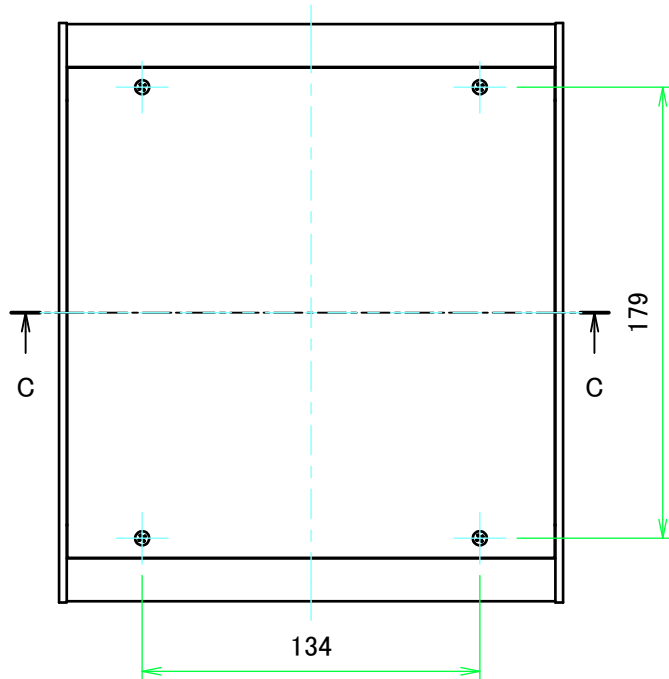
E view
