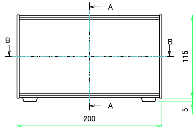
F view
