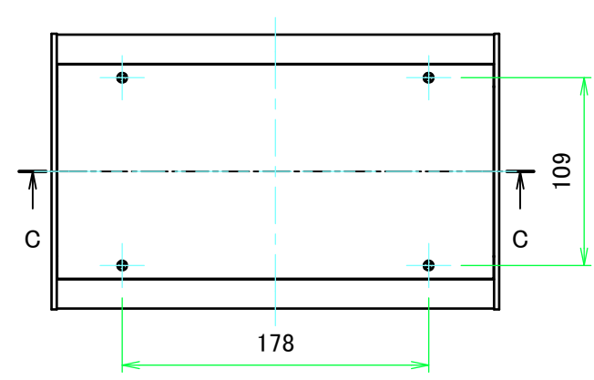
E view
