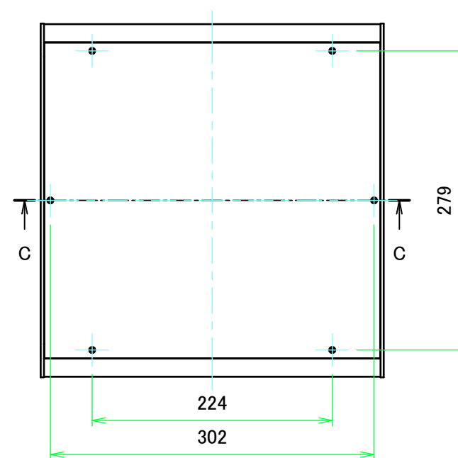
E view
