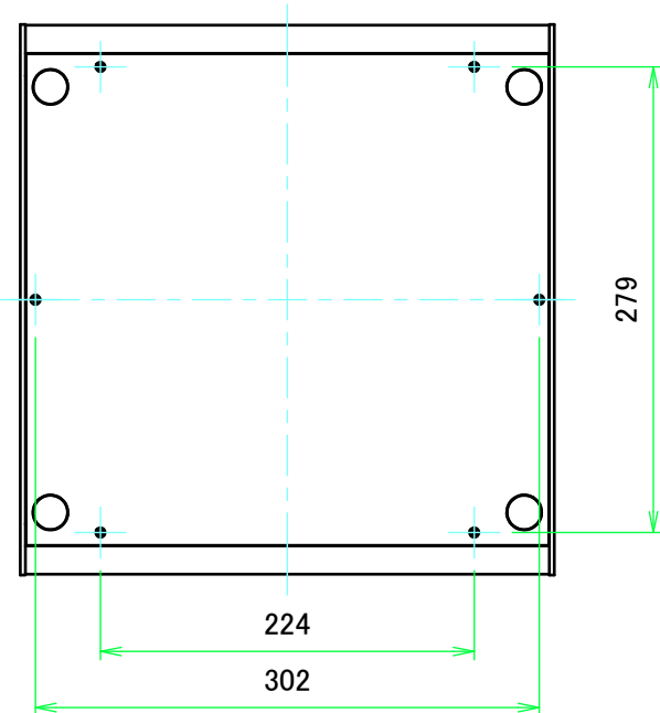
F view
