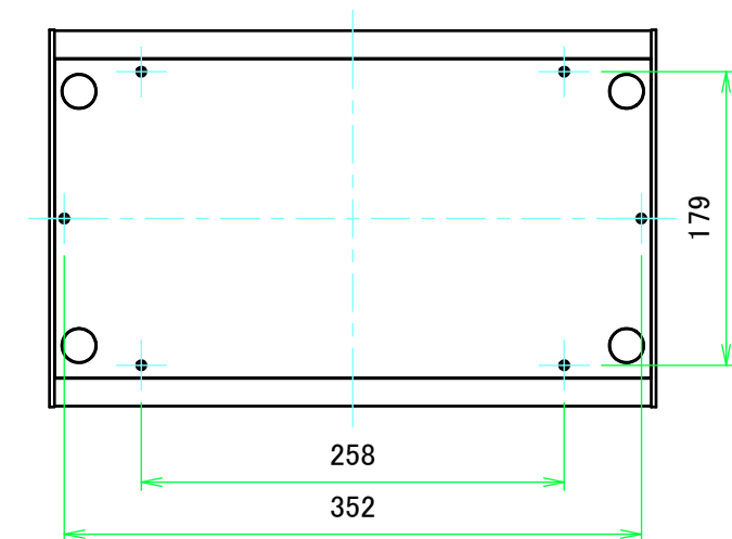
F view
