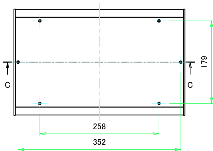
E view
