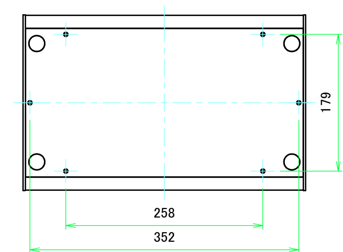
F view
