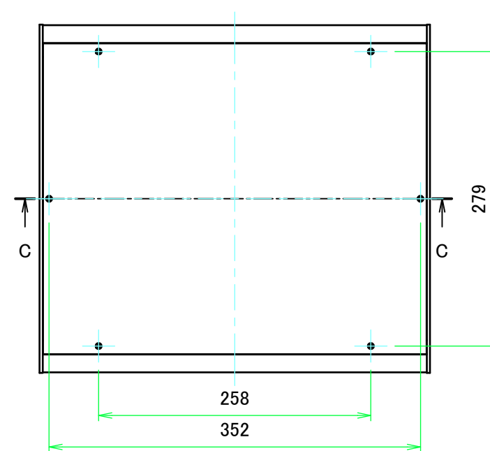
E view
