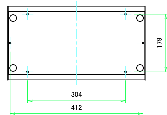
F view
