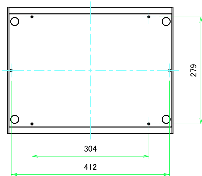
F view
