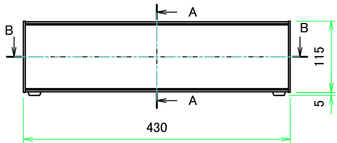
A view
