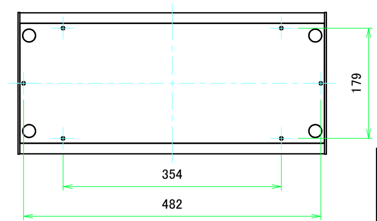
F view
