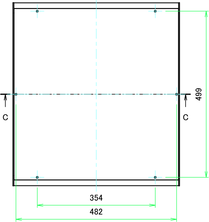
A view
