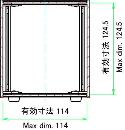
C-C (1:3)
