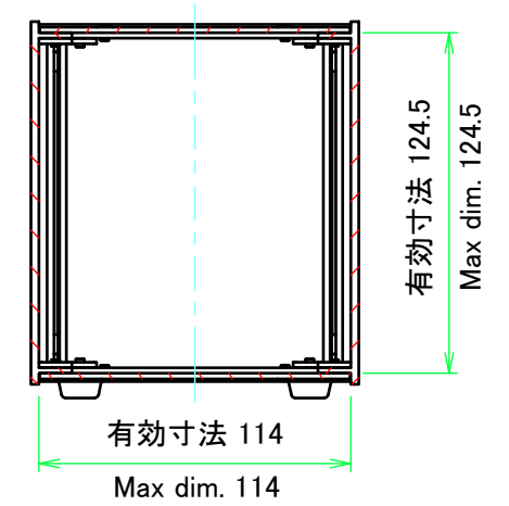
C-C (1:3)
