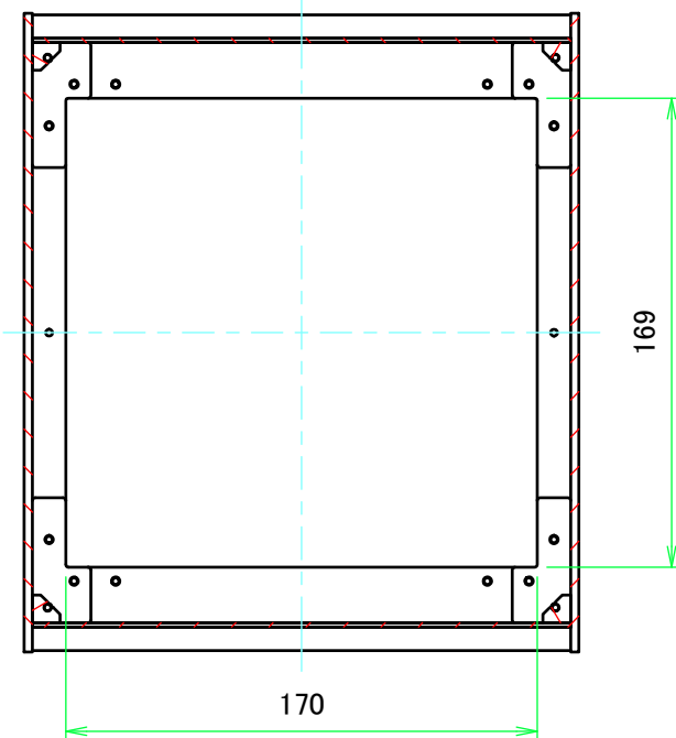
B-B (1:3)
