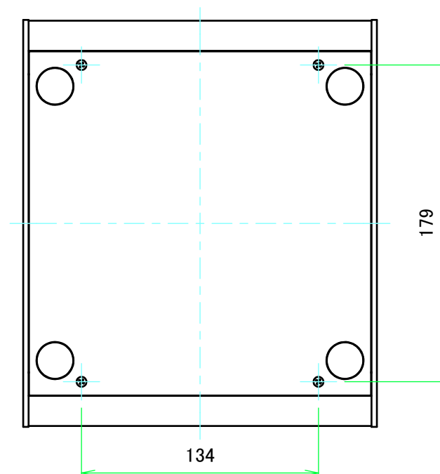
F view
