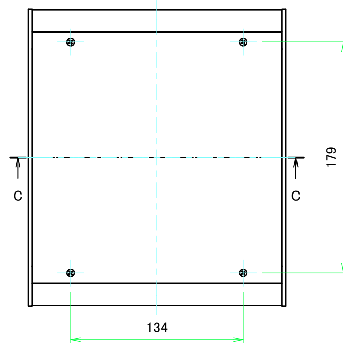
A view
