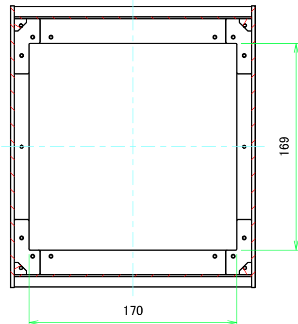
B-B (1:3)
