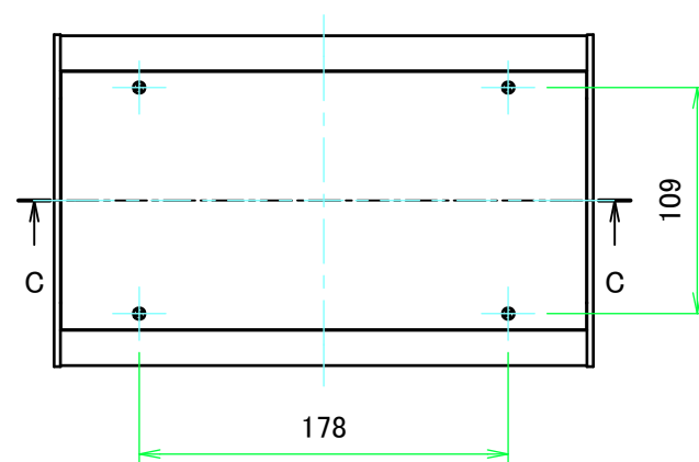
E view
