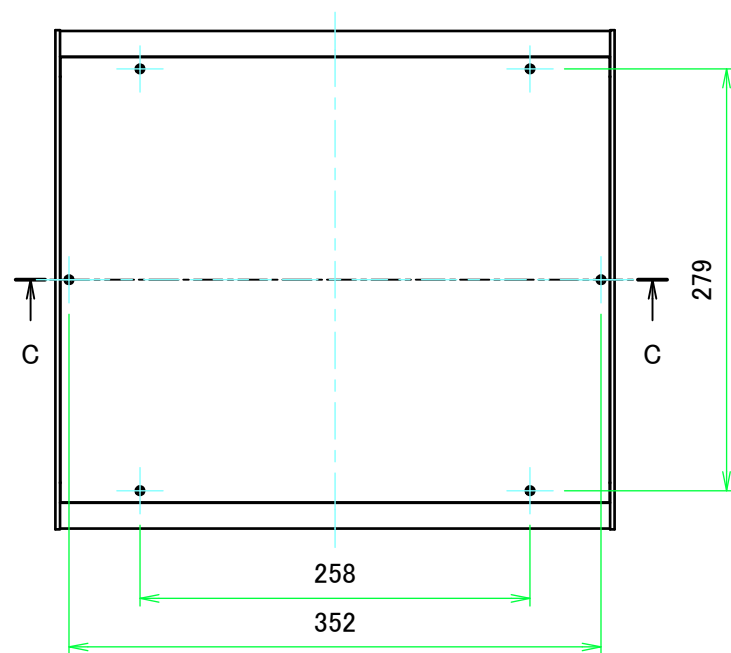
E view
