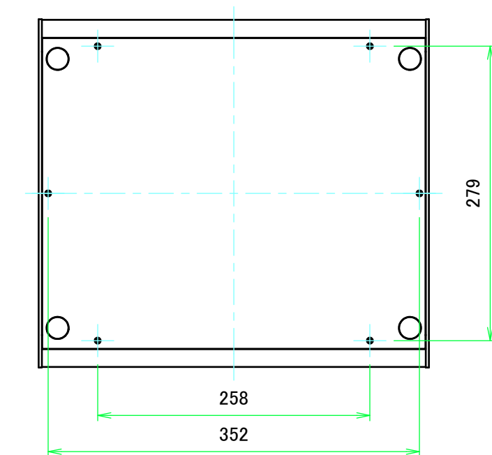
F view
