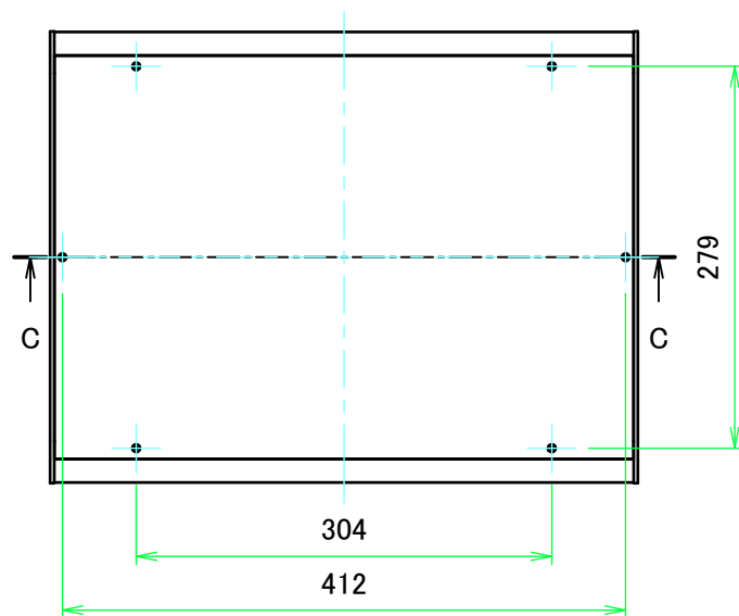
E view
