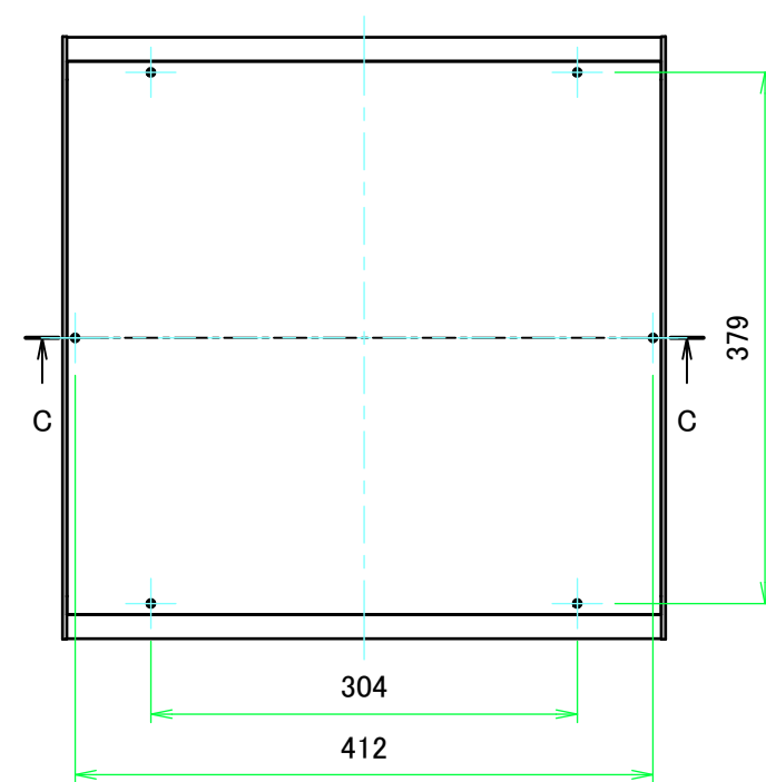
E view
