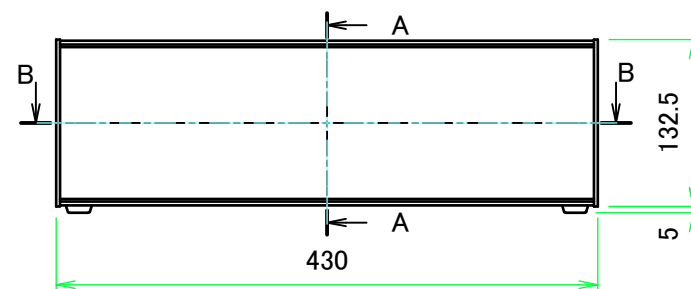
A view
